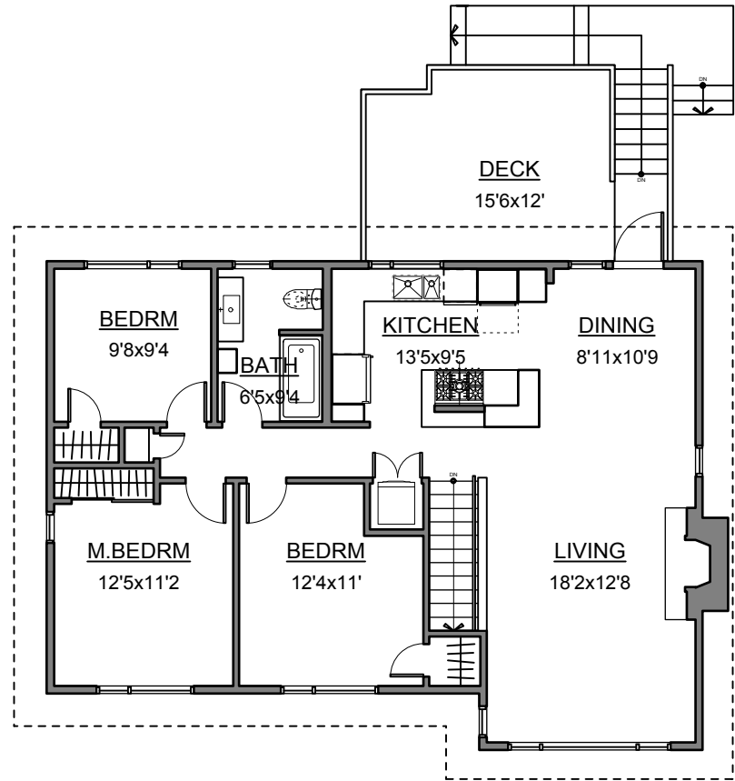
2 UPPER FLOOR PLAN
