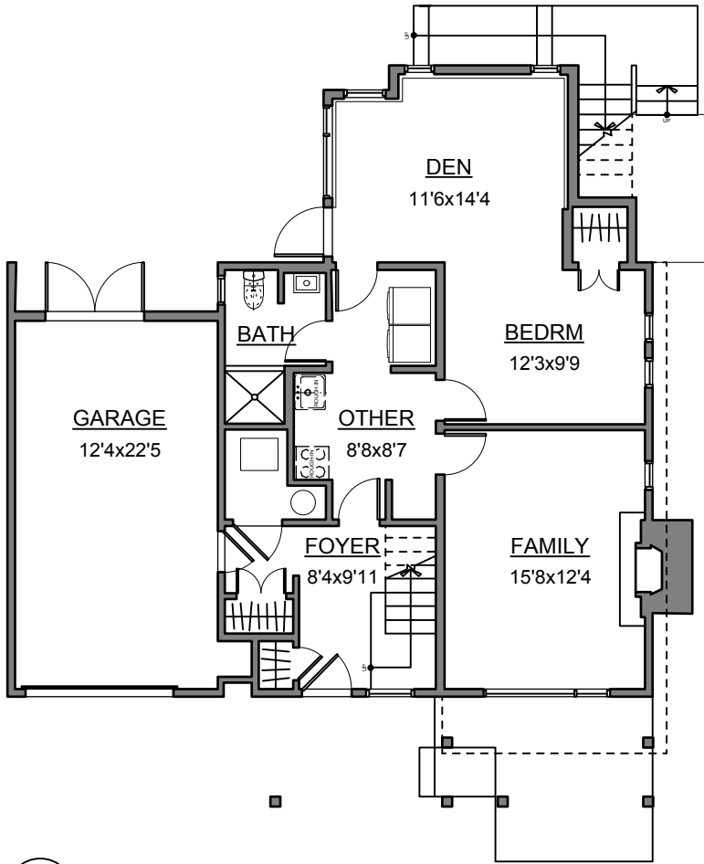
1 GROUND FLOOR PLAN
